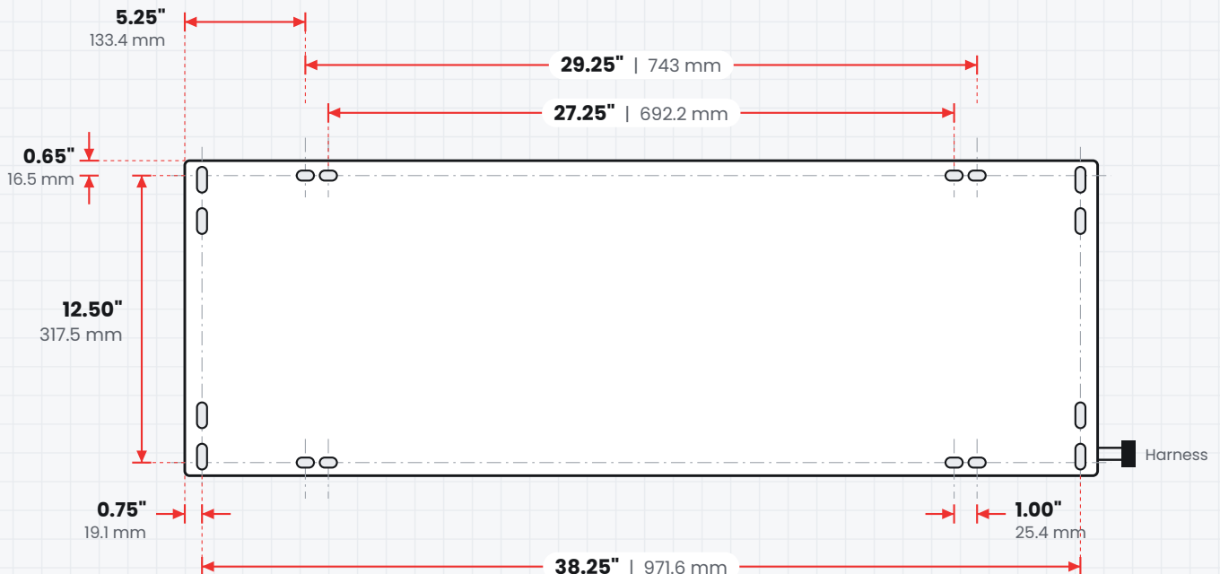
TOP VIEW · MOUNTING PLATE
